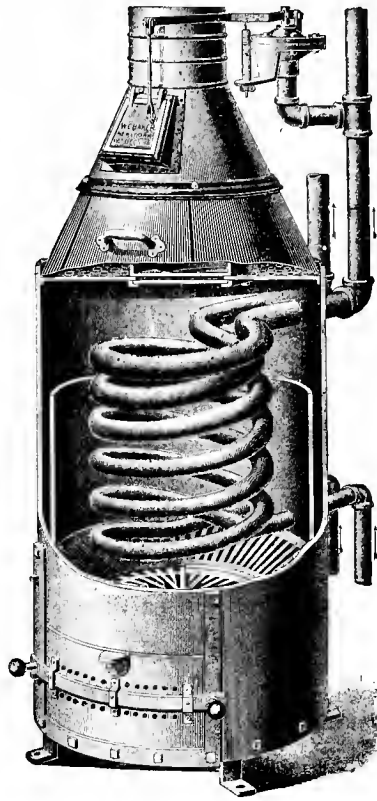
Fig. 2885. Sectional View.
